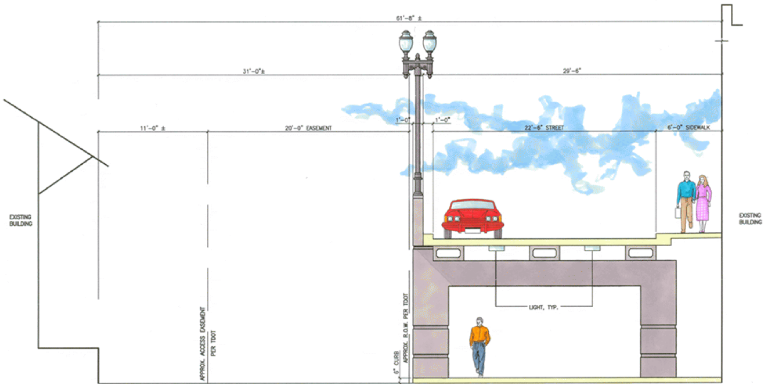
1 SECTION THROUGH JACKSON AVENUE EAST RAMP SD1.4 SCALE: 1/4"=1'-0"
