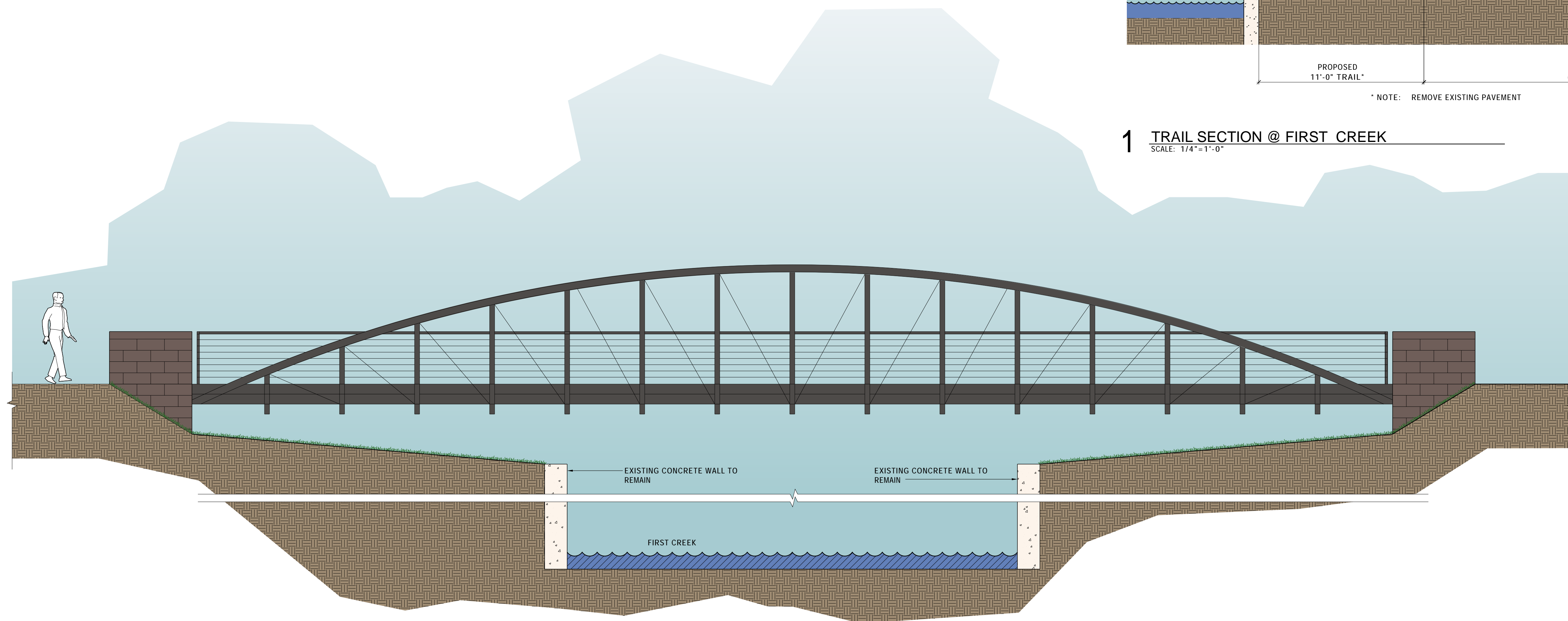
2 TRAIL BRIDGE (80' SPAN) AT FIRST CREEK SCALE: 1/4"=1'-0"
