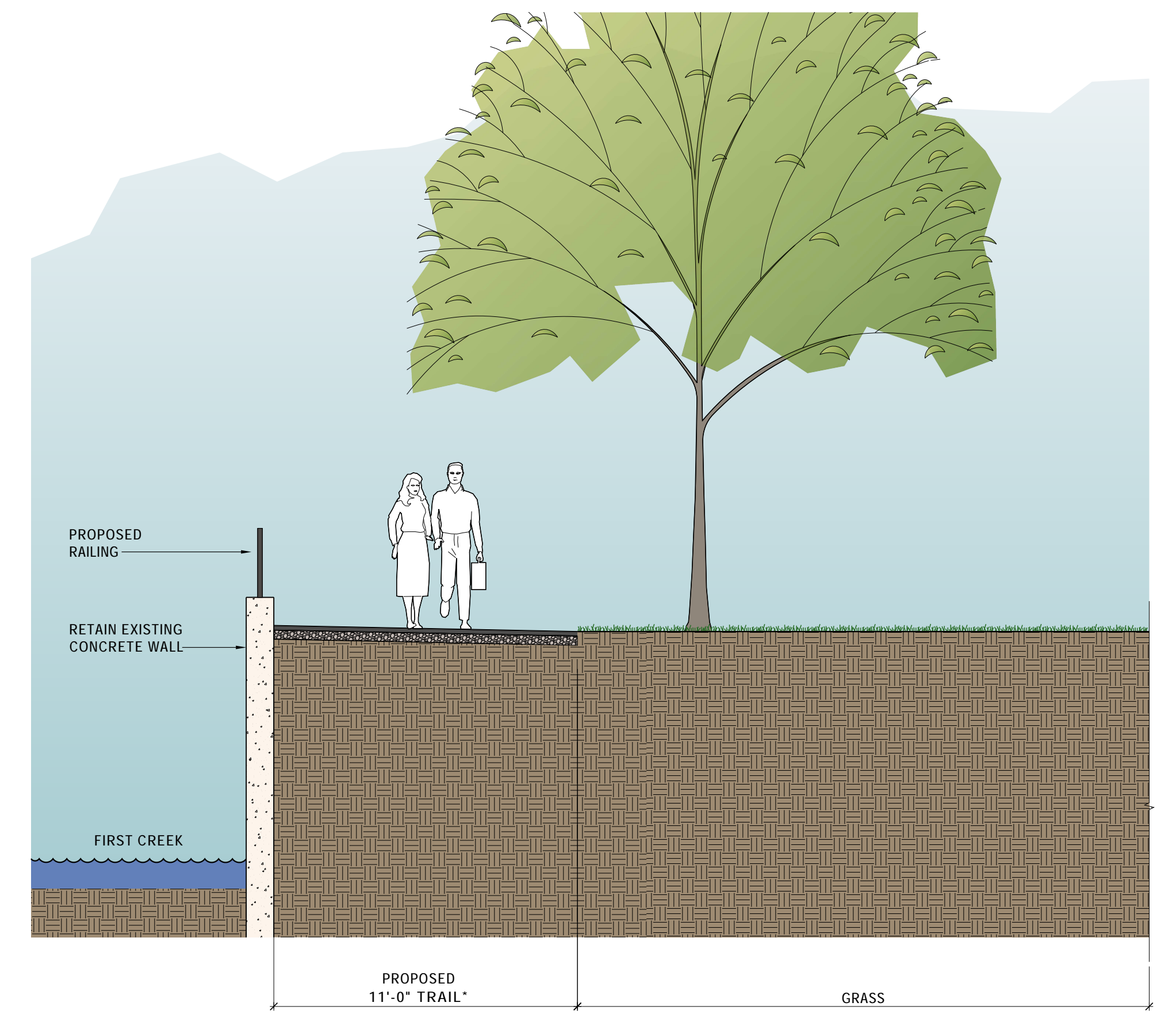
1 TRAIL SECTION @ FIRST CREEK SCALE: 1/4"=1'-0"
